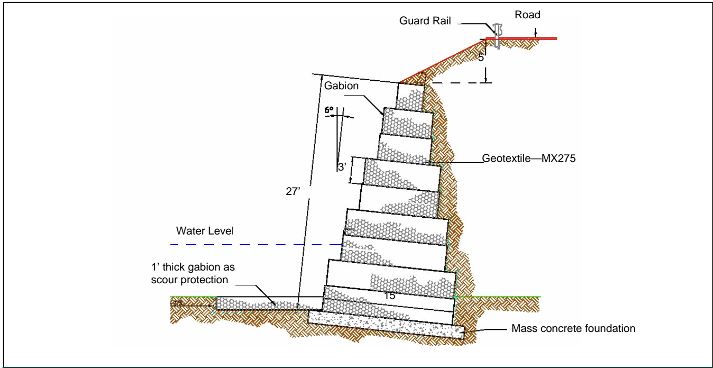
Project section
